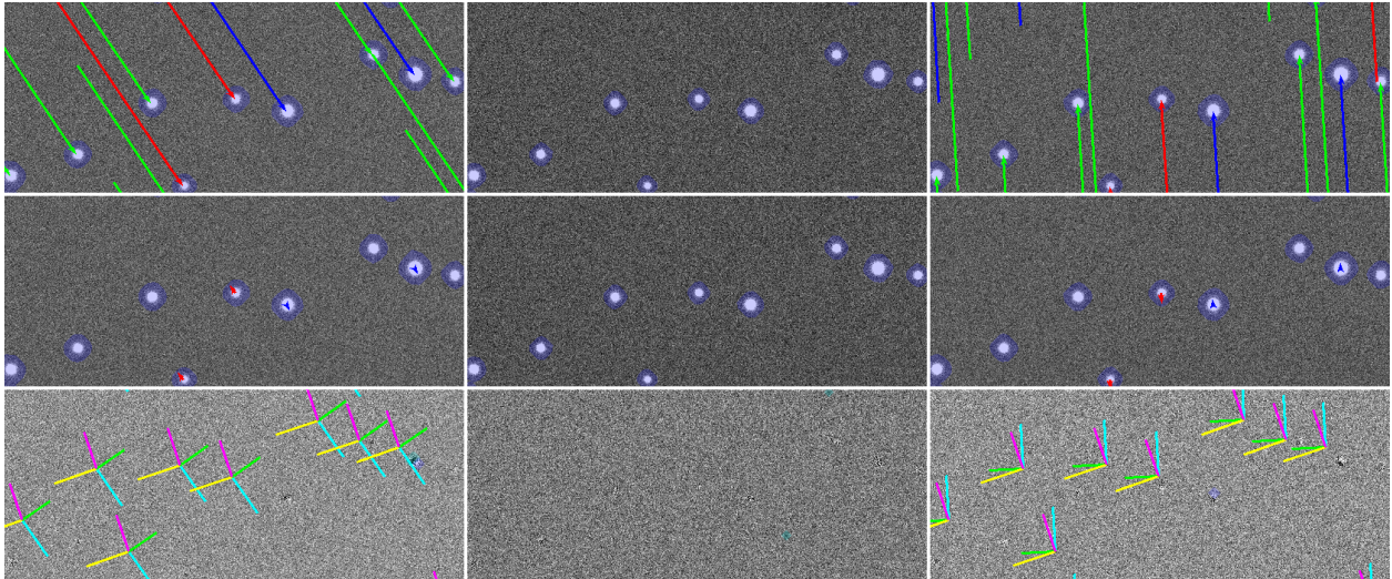
Figure 15: Differential Chromatic Refraction and Difference Image Quality, r -band: Same as Figure 14, but for r -band data. This figure was created using the script python/-compareDcrFromSims.py .
