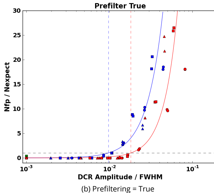
Figure 9: DCR Impact on False Positives: We plot the number of false positives that associate with A0V stars as the blue points, and M2.0V stars as the red points. We normalize by the number expected due to fluctuations in the background, such that y=1 (horizontal black line) represents a doubling of false positives. We plot this value as a function of the measured DCR offset determined via WCS residuals (Table 5), normalized by the FWHM of the PSF. We collapse information from all 3 passbands on this figure; the i -band data tend to have the smaller x -values, and the g -band data larger values. We additionally include information from all 3 seeings by plotting seeing 1 data as circles , seeing 2 as squares , and seeing 3 as triangles . We plot regressions of the form \log_{10} y = a + b \log_{10} x as solid lines, and the positions where these curves cross y=1 as vertical dashed lines. This figure was created using the script python/fpRegressions.py .
