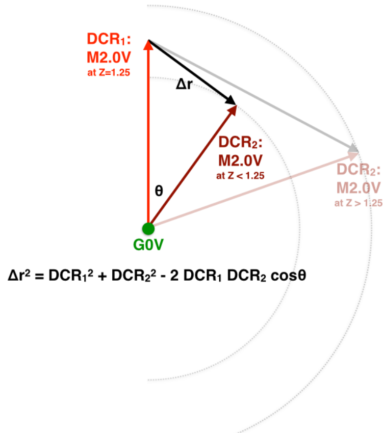
Figure 11: Geometric Basis for Figure 12: This figure provides the geometric basis for the study of astrometric offsets induced by DCR, as a function of difference in airmass and parallactic angle, for a single SED. We use a reference DCR amplitude for the basis of this study, labeled here as DCR1 and representing the DCR of the M2.0V star at 1.25 airmasses with respect to the G0V star. A second observation of this object is labeled DCR2, and is observed at a different airmass (representing a different DCR amplitude, plotted along the y-axis in Figure 12) and parallactic angle (denoted by theta, plotted along the x-axis in Figure 12) than the reference observation. The law of cosines is used to find the amplitude of the DCR offset \Delta r , which is used to color-code the panels in Figure 12. The distance \Delta r is effectively the distance from point DCR1 to the perimeter of the circle whose radius is DCR2.
