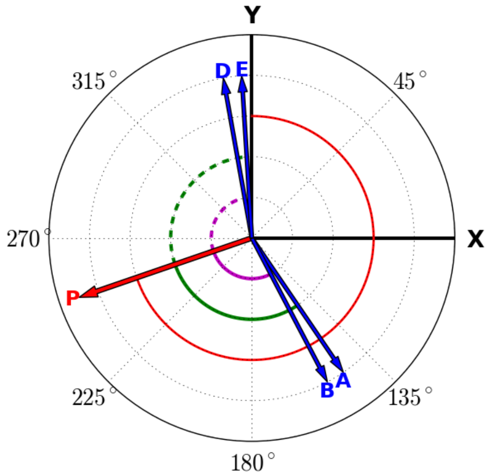
Figure 5: Designed Orientation of DCR in W14 PhoSim Runs: This figure represents the anticipated orientations of DCR in the W14 phoSim data. The x,y coordinate system is depicted, as well as the convention that angles ( rotTelPos , rotSkyPos ) rotate clockwise with respect to the positive y -axis in the image coordinate system (and counterclockwise in the camera coordinate system). The rotTelPos of 251 degrees specified for all simulations, which reflects the direction to the pole, is shown with the red vector P and the red arc at y=0.6 . The derived rotSkyPos for visits A,B,D,E are shown with the blue vectors, and reflect the angle towards zenith (the angle of increasing altitude). DCR is expected to happen along these vectors. The angles PA,PE are similar, and represented by the green arcs at y=0.4 ; the angles PB,PD are also similar, and represented by the purple arcs at y=0.2 . This is expected as observations A and E are taken at airmass 1.55 (zenith distance of 50 degrees) but at opposite sides of the meridian crossing of the star field; a similar situation was designed for observations B and D , which are taken at airmass 1.16 (zenith distance of 30 degrees). Visit C is not depicted as it was taken at zenith. This figure was created using the script python/dcrSchematic.py .
