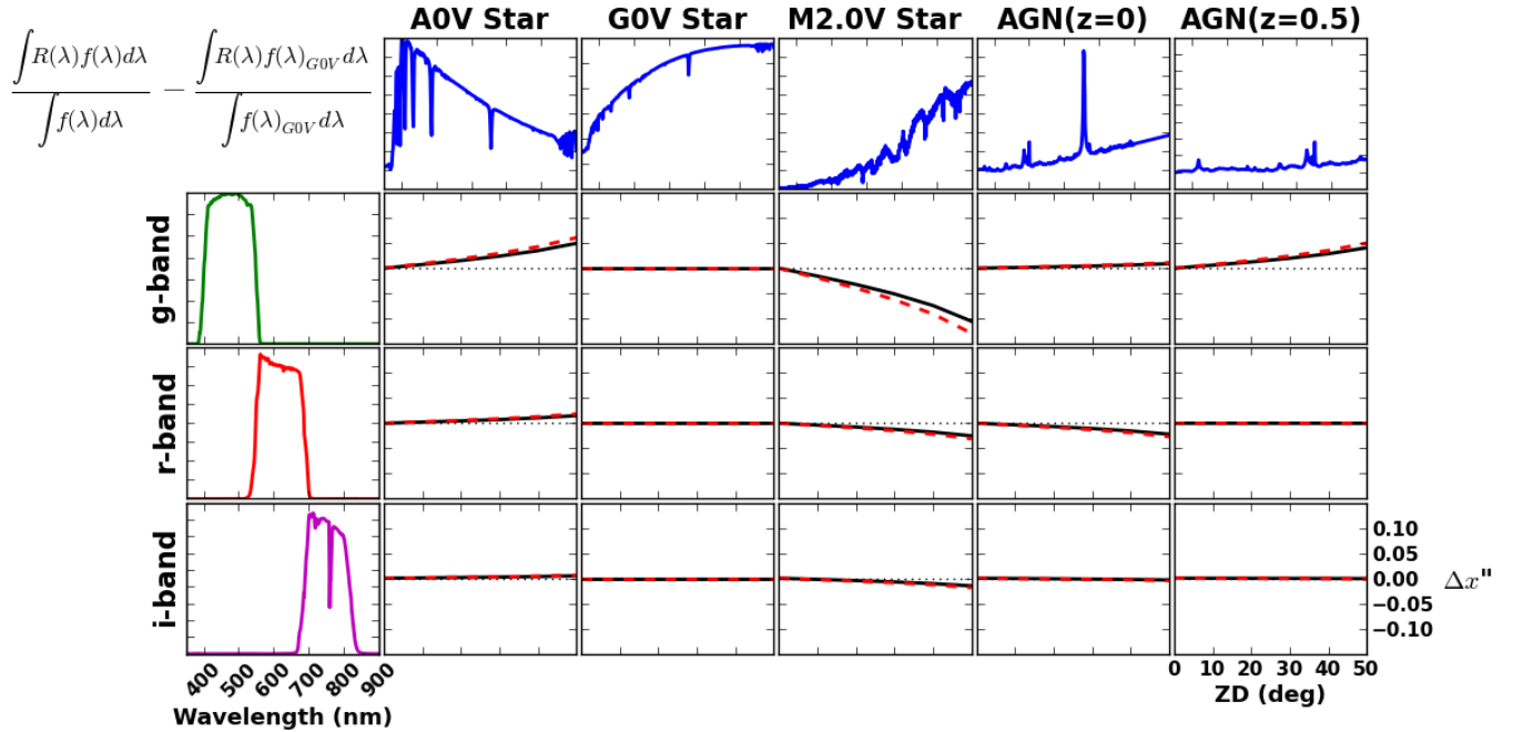
Figure 3: Differential Chromatic Refraction vs. Filter and Spectral Energy Distribution:
