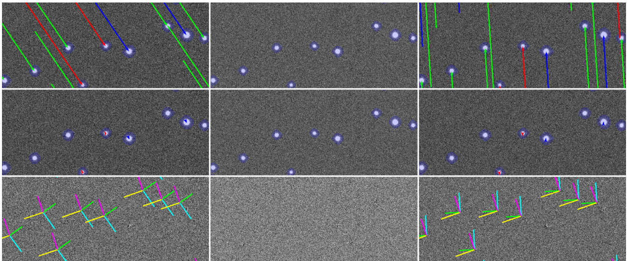
Figure 16: Differential Chromatic Refraction and Difference Image Quality, i -band: Same as Figure 14, but for i -band data. This figure was created using the script python/compareDcr-FromSims.py .
