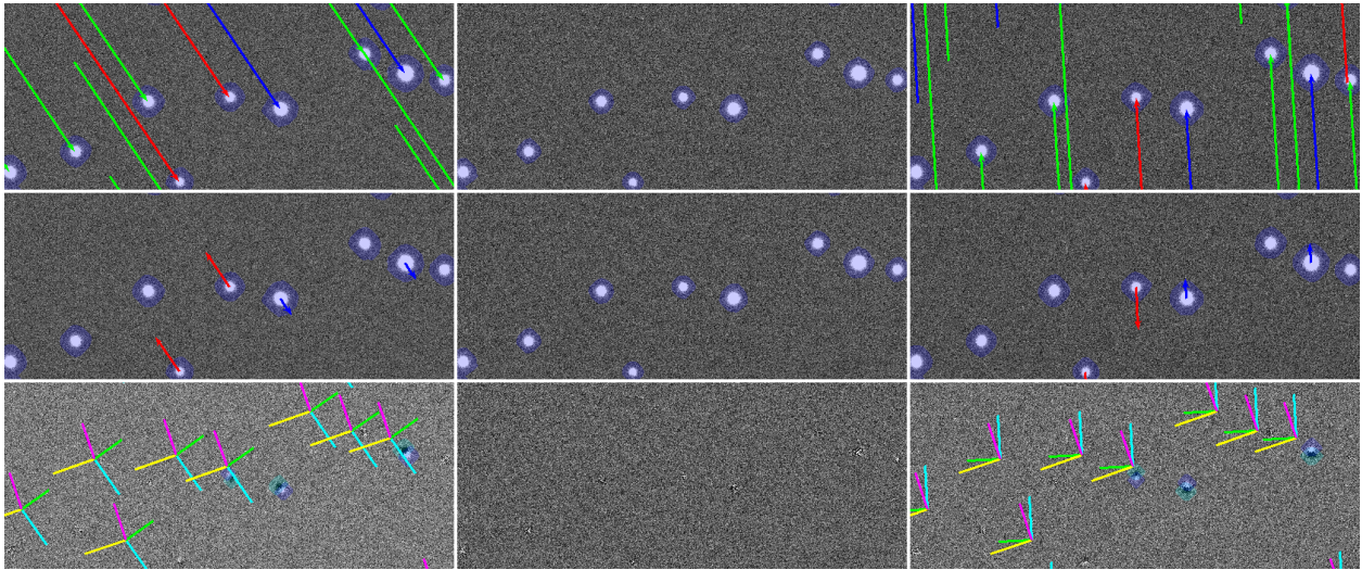
Figure 14: Differential Chromatic Refraction and Difference Image Quality, g -band: This set of panels demonstrates the amount of refraction (top row), differential refraction with respect to the G0V star (middle row), and the quality of the difference image (bottom row) for three sets of image differences. The first column uses science visit A, the middle C, and the third E. In all cases the template used was taken at zenith, i.e. visit C. The top rows effectively present the same information as Figure 13, but zoomed in on a particular cluster of stars. The second row subtracts off the green vector from all vectors. The residual refraction of the blue, red vectors represents differential chromatic refraction. These residual lengths have been multiplied by a factor of 100 for readability. Note that the blue vectors point along the vector to zenith, indicating the blue stars appear higher in the sky than their green counterparts, compared to an unrefracted observation. The red stars are not refracted as much and thus will appear lower in the sky. On the bottom row, we show the realized difference image quality. Note that the blue stars have positive lobes pointing along the direction to zenith, meaning the stars are “higher” in the sky w.r.t. the green stars when compared to the zenith template, while the dipoles of the red stars have the opposite polarity. For completeness, the Wcs-derived orientation of the Ra, Dec and Az, Alt coordinate axes are shown in the difference image (Ra, Dec, Az, Alt are magenta, yellow, green, cyan); see Figure 6 for more detail. This figure was created using the script python/compareDcrFromSims.py .
