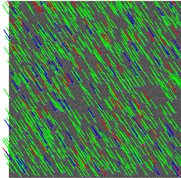
Figure 13: Refraction: This figure depicts the amplitude and orientation of the refraction vector in the visit A, raft=2,2 sensor=1,1 filter=g, seeing value 2 data. The vectors point from the unrefracted locations to the realized locations in the image. The SEDs of the sources are indicated with colors blue, green and red for A0V, G0V, and M2.0V respectively. This figure was created using the script python/compareDcrFromSims.py.
