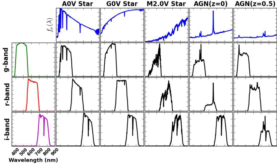
Figure 1: Effective Spectral Energy Distributions : The effective spectra of 5 reference objects – a “blue” A0V, a reference G0V, and a “red” M2.0V star, along with a QSO at redshift z = 0 and z = 0.5 – filtered through 3 transmission profiles corresponding to the LSST g , r , and i -bands at 1.2 airmasses. The top row shows the input spectral energy distribution f_v(\lambda) , while the leftmost column shows the LSST filter transmission profile in units of the normalized system response \phi . The inner row, column figures show the effective spectrum of each SED (along columns) when multiplied through the respective filter (along rows). In all subpanels, the x-axis is wavelength. The A0V, G0V, and M2.0V spectra correspond to CAT_SHARE_DATA files kp01_9750.fits_g45_9830.gz, km20_6000.fits_g30_6020.gz, and m2.0Full.dat.gz respectively, and were used as the SEDs of the stars in the W14 image simulations. This figure may be recreated using the script python/DCR.py.
